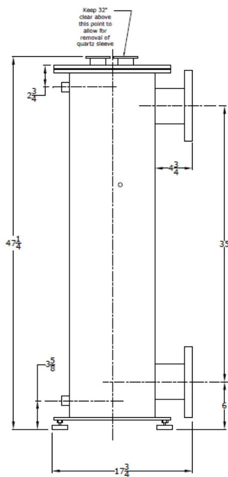
Chamber "U" shape
