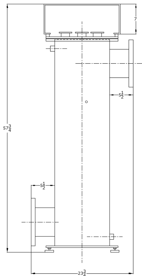
Chamber "Z" shape
