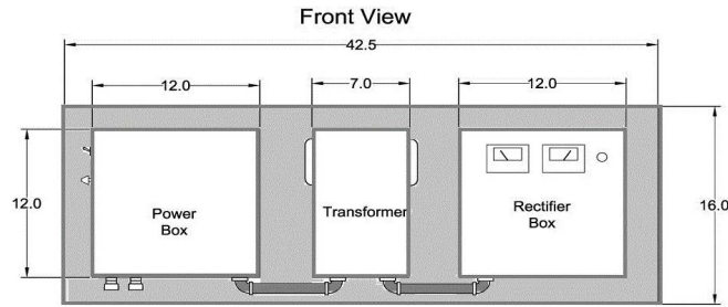
Horizontal power supply
